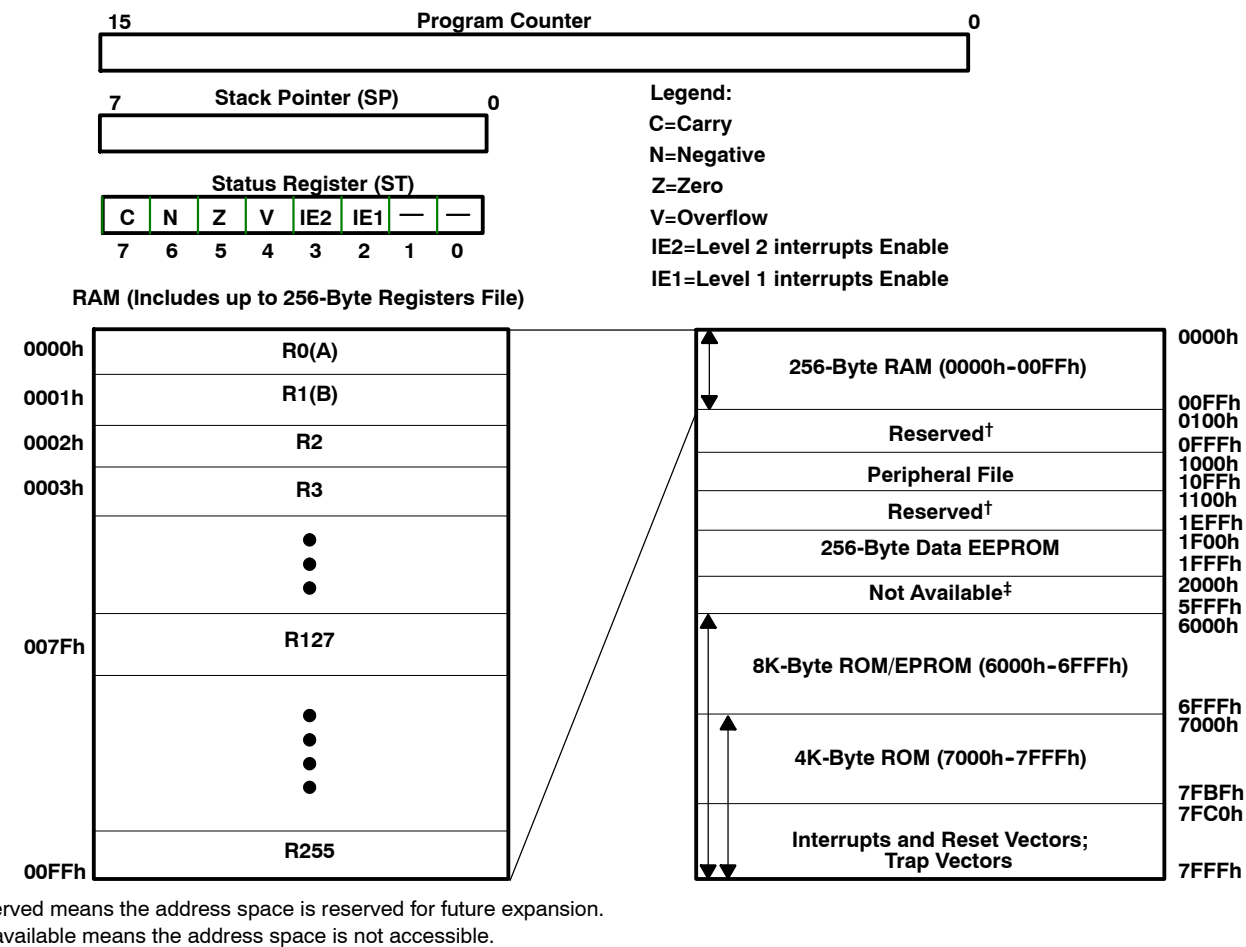
Figure 1. Programmer's Model
